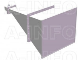
LB-340-20-C-SFSPO Standard Gain Horn Antenna 2.2-3.3GHz 20dB Gain SMA Female
