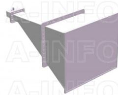
LB-340-20-C-NFSPO Standard Gain Horn Antenna 2.2-3.3GHz 20dB Gain N Type Female
